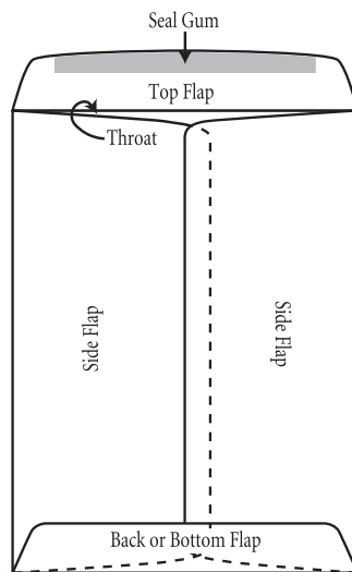
Open End, Center Seam
